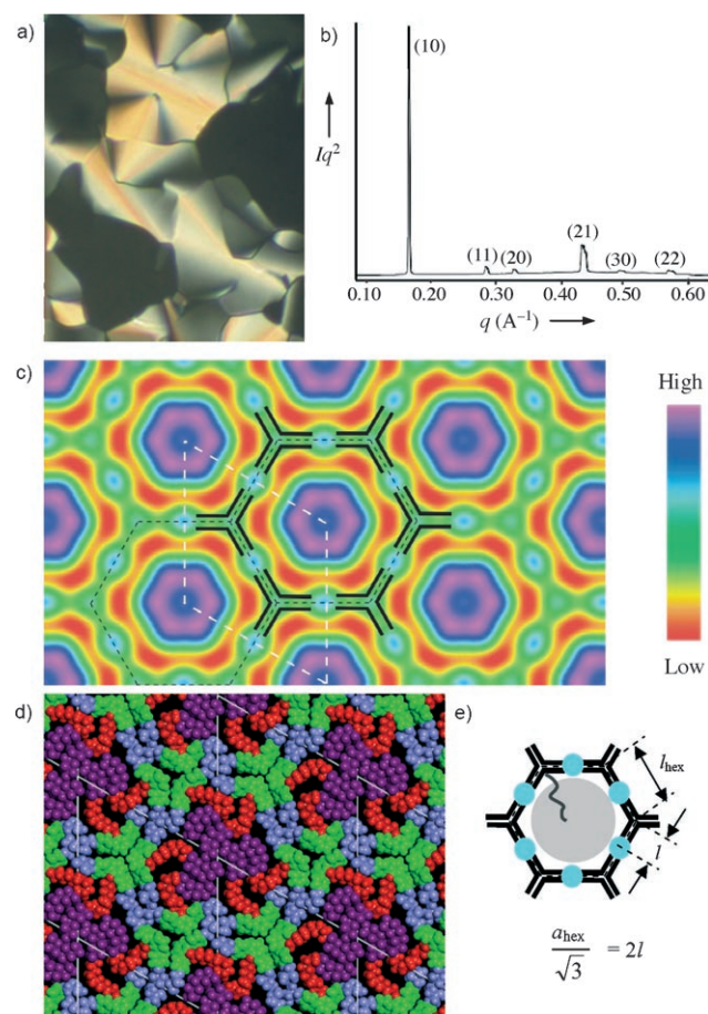
Figure 1. Col hex /p6mm phase of compound 1c : a) texture between crossed polarizers at T = 135^\circ\text{C} ; b) X-ray diffraction pattern (small angle region) at 127^\circ\text{C} ; c) reconstructed electron density map. See text for details and color coding; d) snapshot of a molecular dynamics simulation (for easy comparison the color coding is the same as in (c)); e) model of molecular organization; blue circles represent hydrogen bonding networks of glycerol groups, black wavy lines represent semiperfluorinated chains; c–e) viewed along the cylinder axis.
